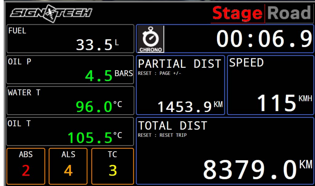
Tripmaster (option)
