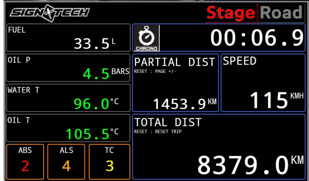
Tripmaster (option)
