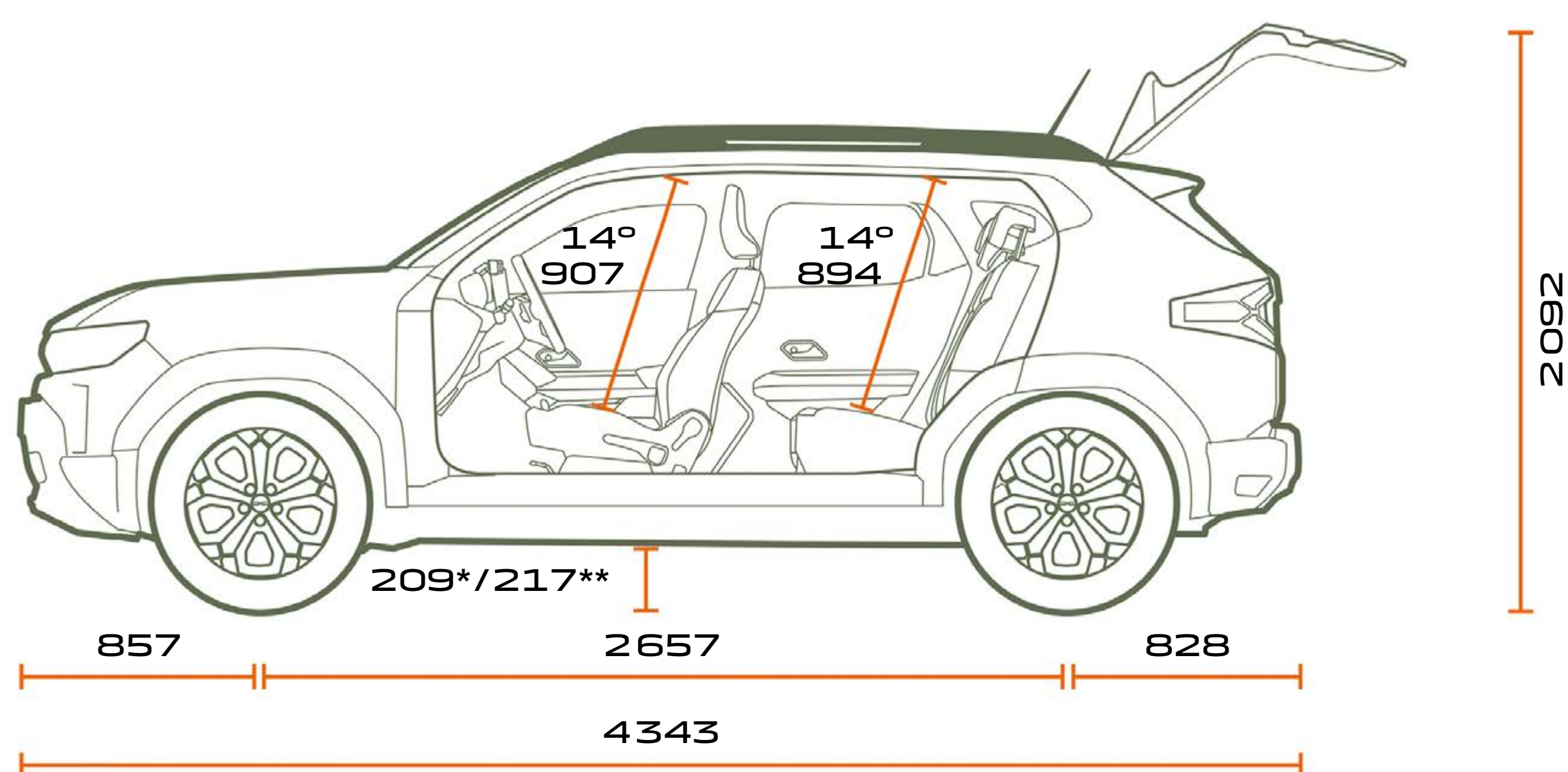
PROFILE VIEW
