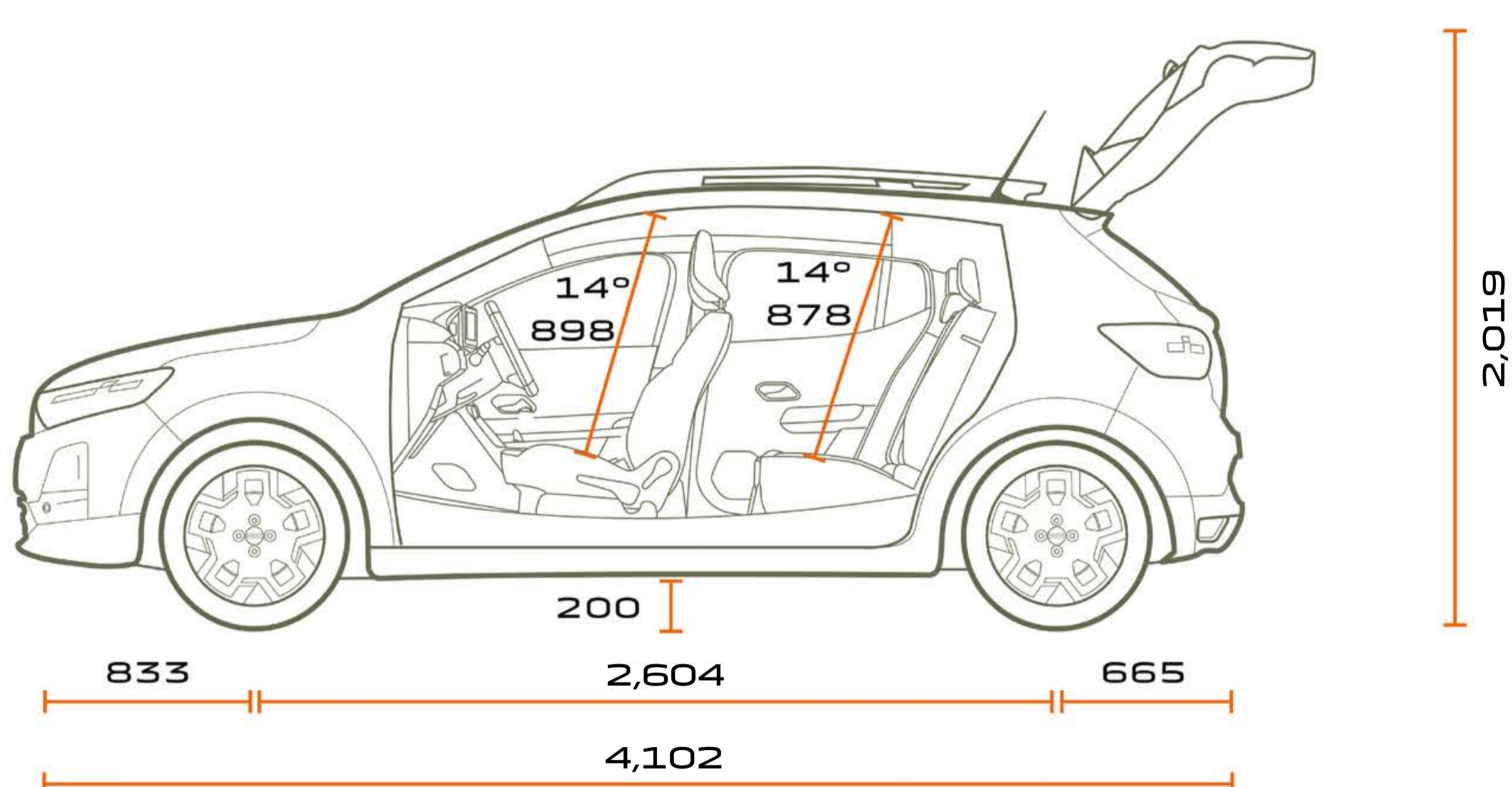
SIDE VIEW
