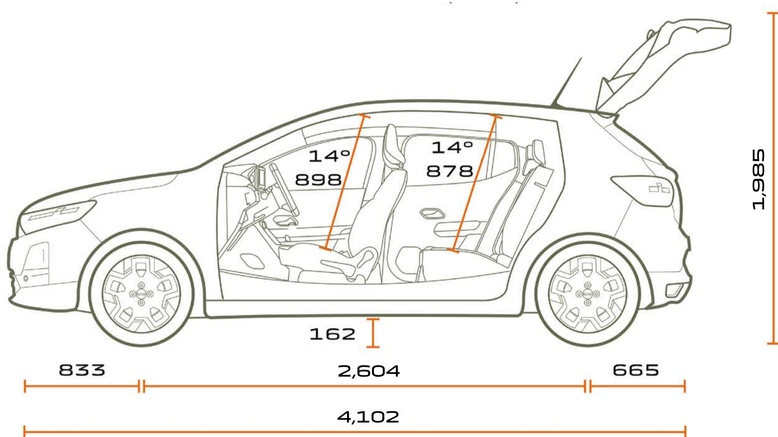
SIDE VIEW
