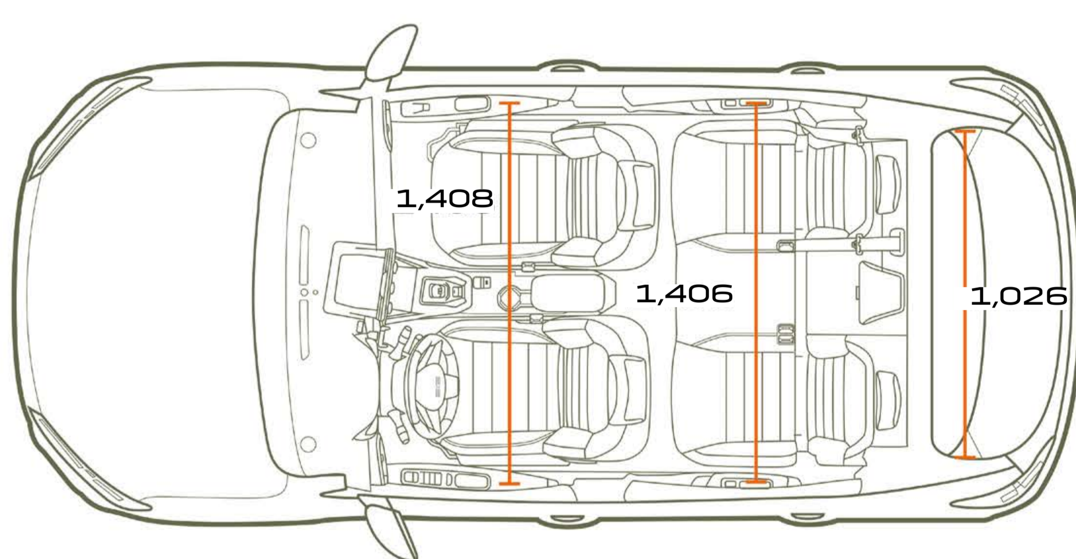
TOP VIEW
