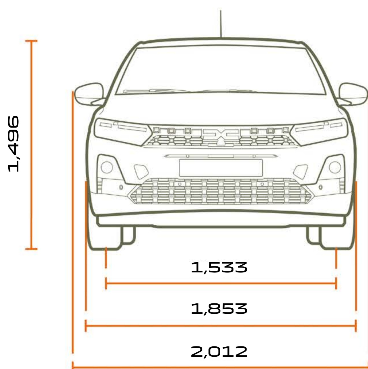
FRONT VIEW
