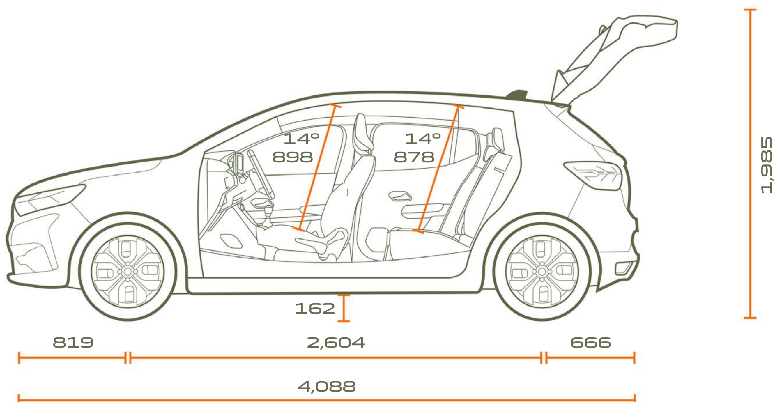
SIDE-FACE VIEW
