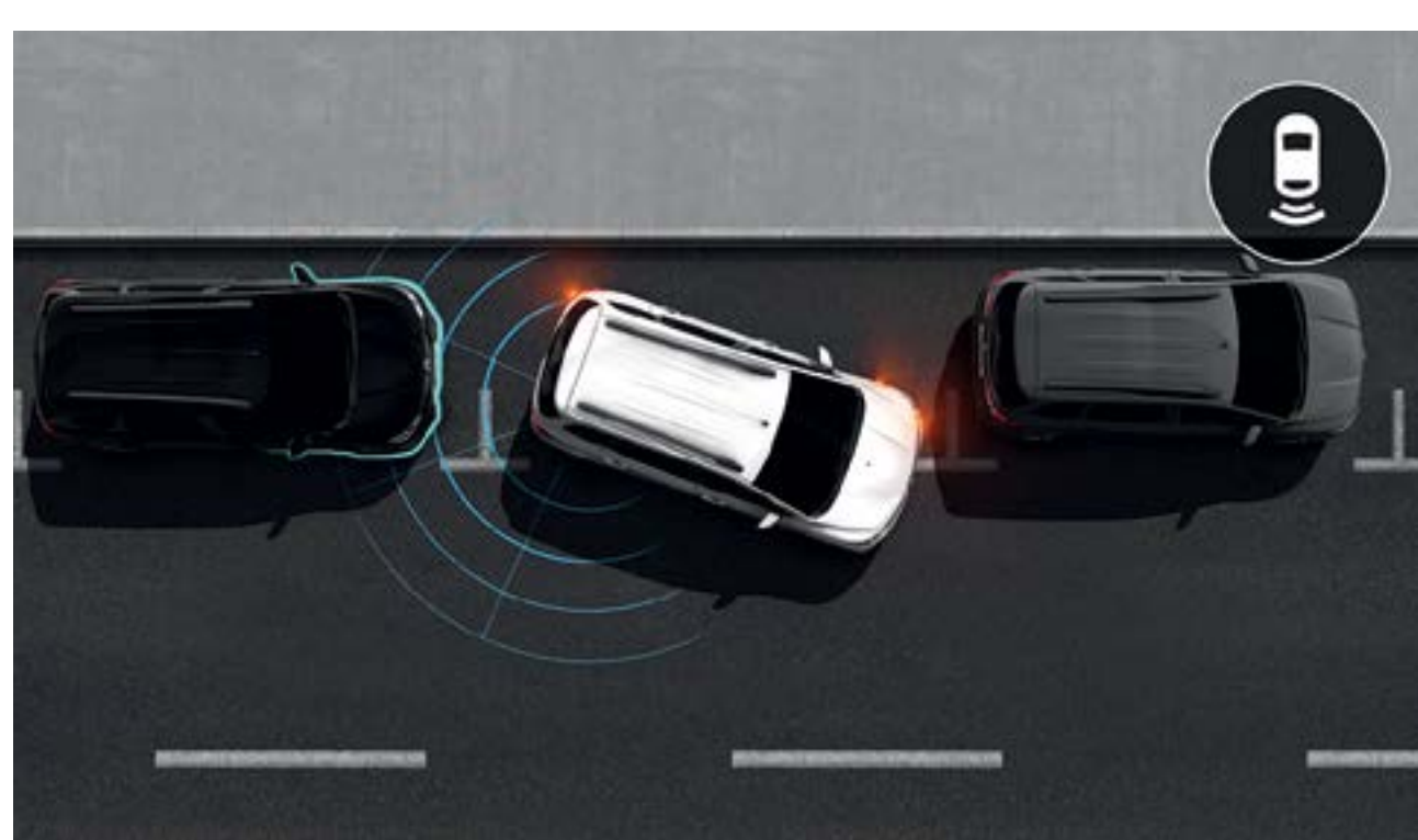
reverse parking sensor Ultrasonic sensors in the rear bumper measure the distance between the vehicle and an obstacle.
