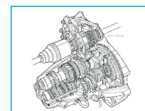
Transmission
