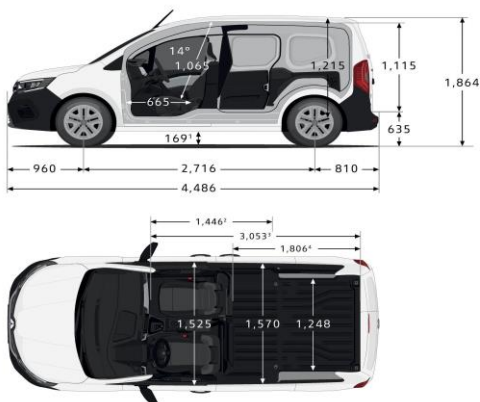
Dimensions (mm)
